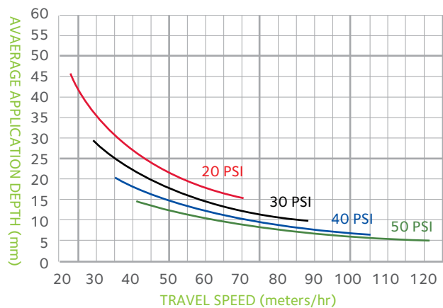
250 & 300 Travelling Irrigator Performance Curves
